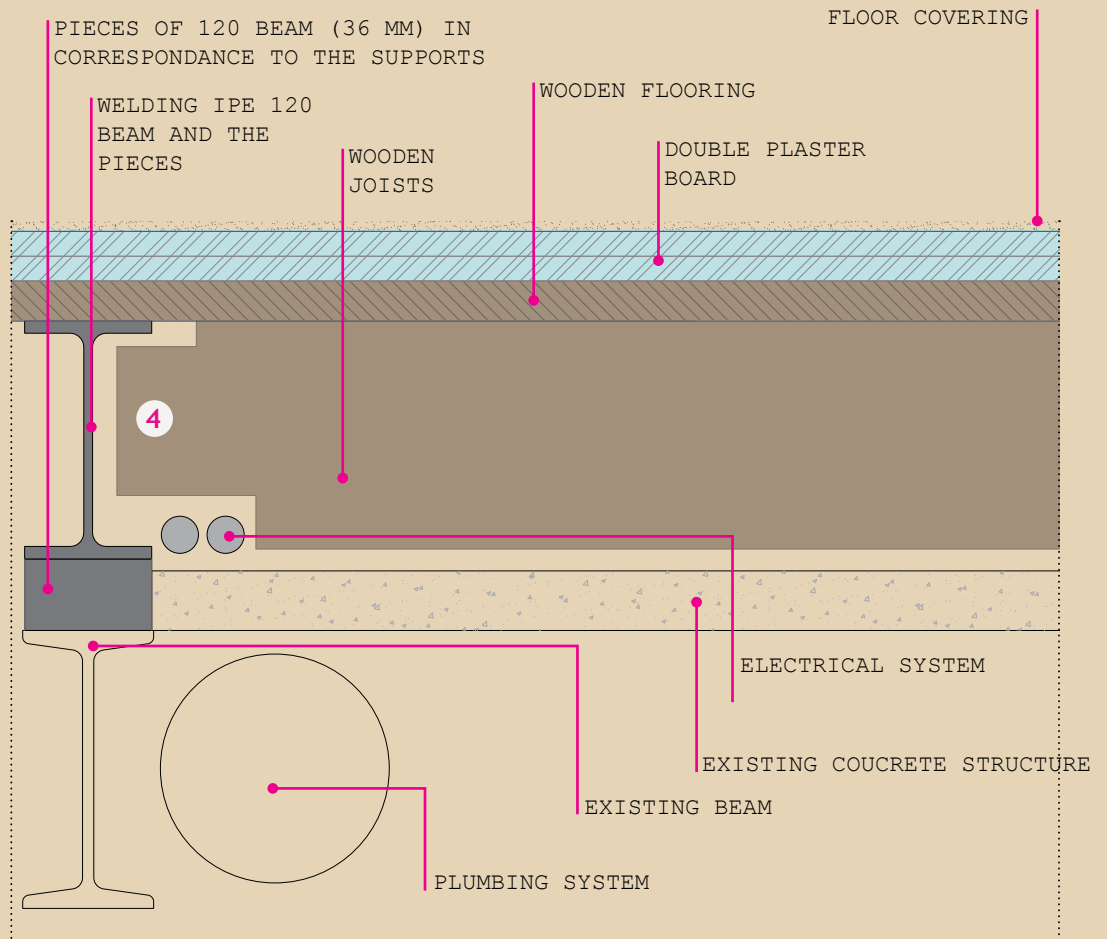
3 FITTING WITH WOODEN JOISTS AND THE IPE
